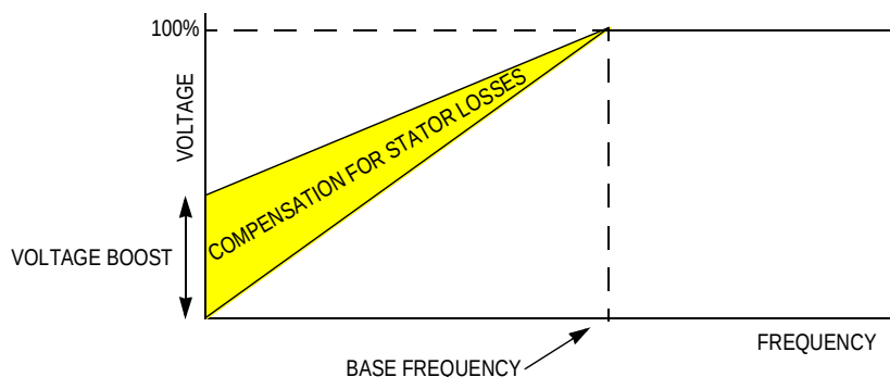
Figure 5. Voltage Profiling, Including Voltage Boost
