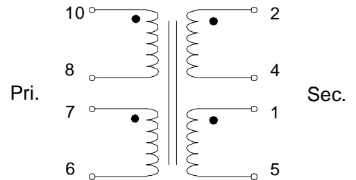
Schematic Diagram
