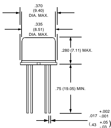
External Dimensions
