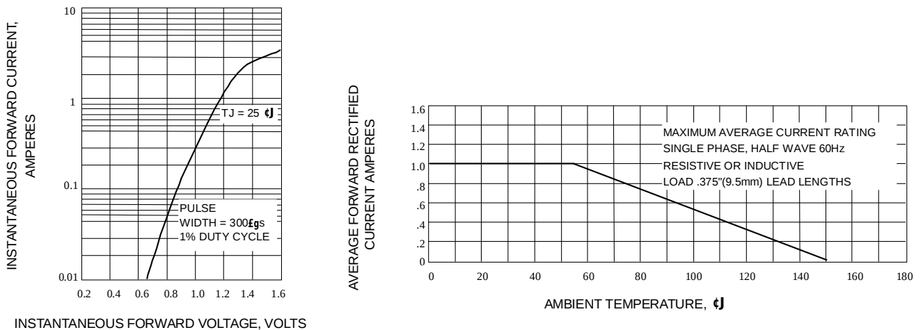
Fig. 2-TYPICAL INSTANTANEOUS FORWARD CHARACTERISTICS
