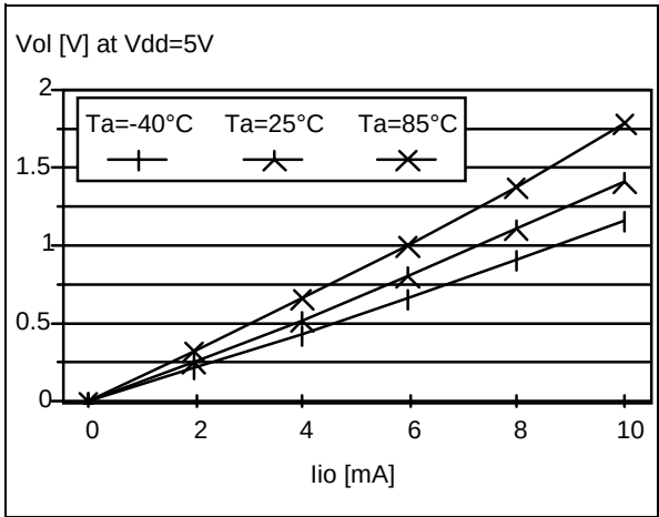
Figure 84. Typical V_{OL} at V_{DD}=5\text{V} (high-sink)
