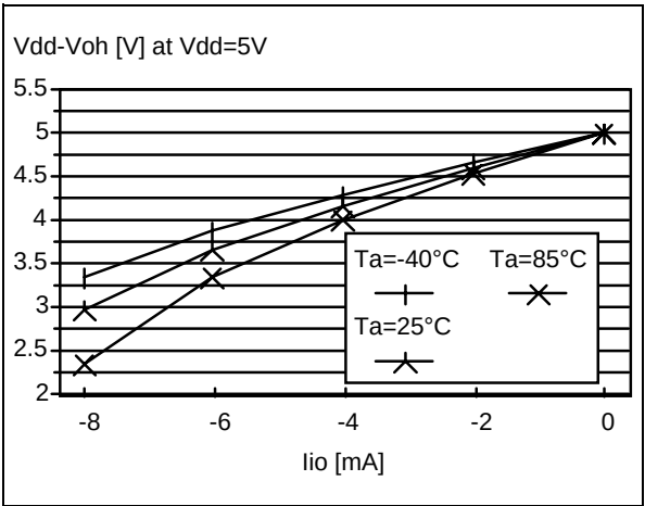
Figure 85. Typical V_{DD}-V_{OH} at V_{DD}=5\text{V}
