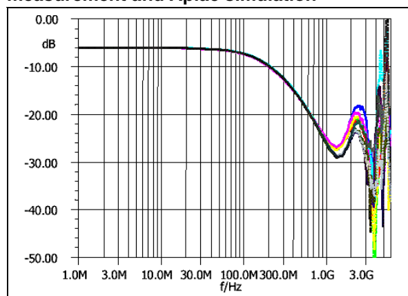
Figure 3: S21(dB) all lines attenuation measurement and Aplan simulation
