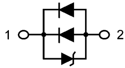
Fig. 13.1 Internal Circuit
