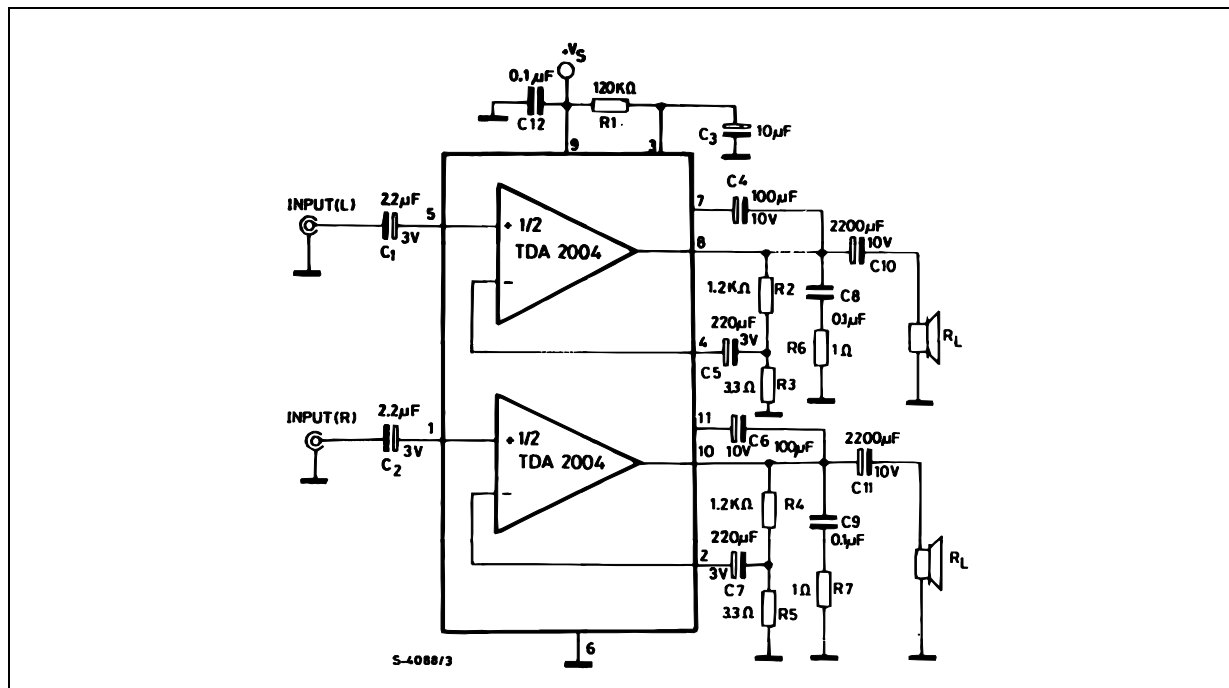
Figure 1 : Test and Application Circuit.
