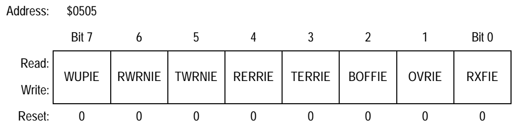
Figure 20-20. Receiver Interrupt Enable Register (CRIER)
