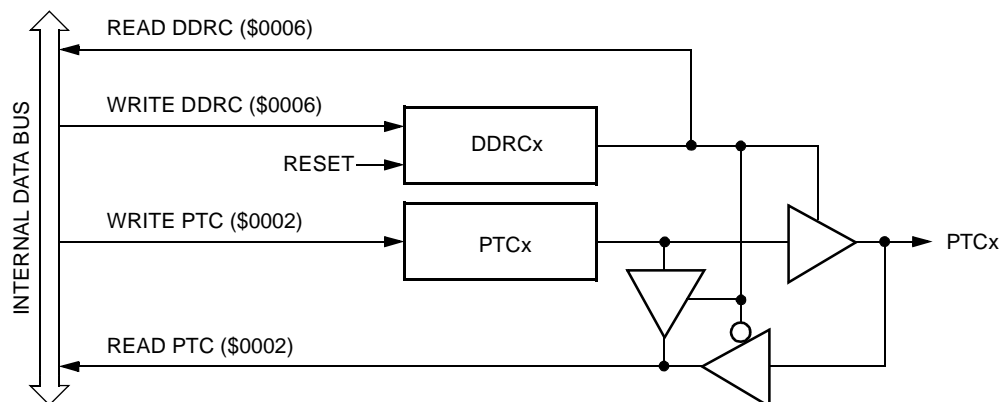
Figure 19-9. Port C I/O Circuit
