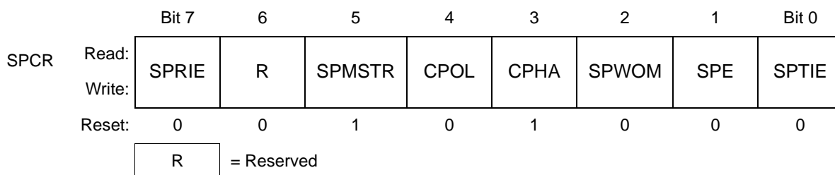
Figure 16-12. SPI Control Register (SPCR)
