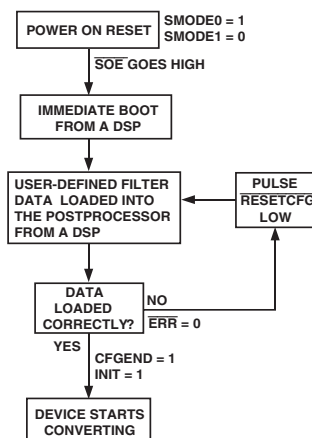
Figure 27. Flow Chart of DSP Mode
