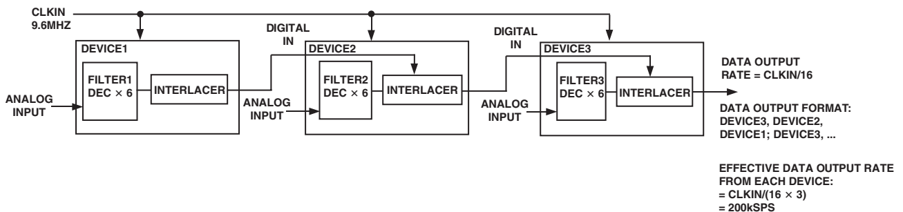
Figure 32. Daisy-Chaining Example
