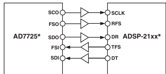
Figure 35. AD7725 to ADSP-21xx Interface
