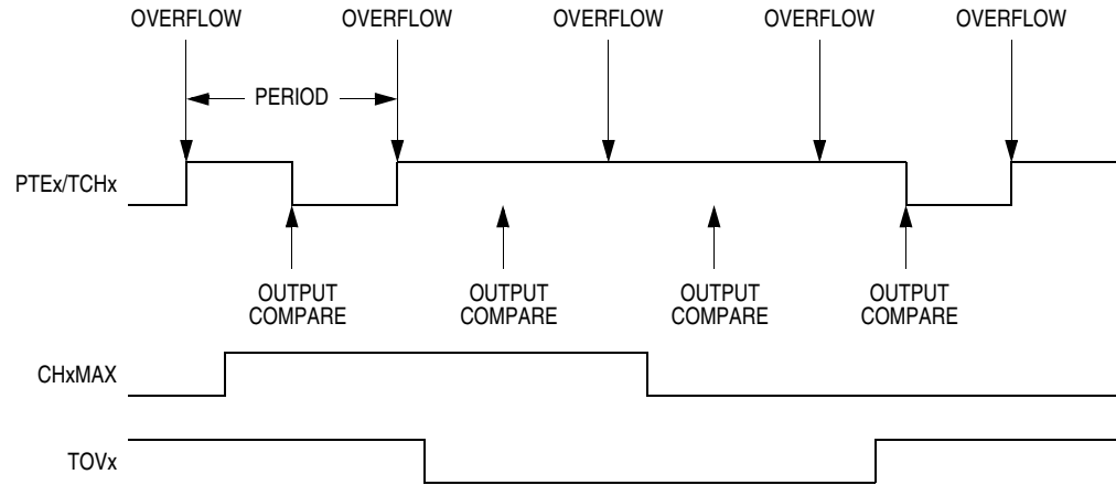
Figure 16-9. CHxMAX Latency
