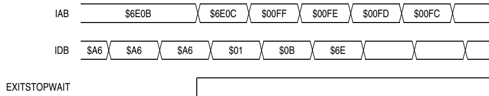
Figure 14-12. Wait Recovery from Interrupt
