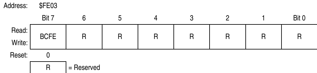
Figure 18-7. SIM Break Flag Control Register (SBFCR)
