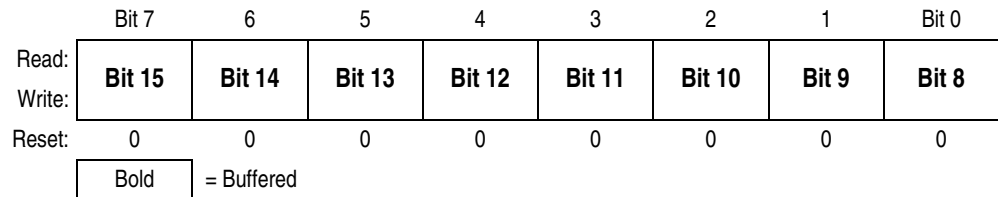
Figure 12-37. PWMx Value Registers High (PVALxH)
