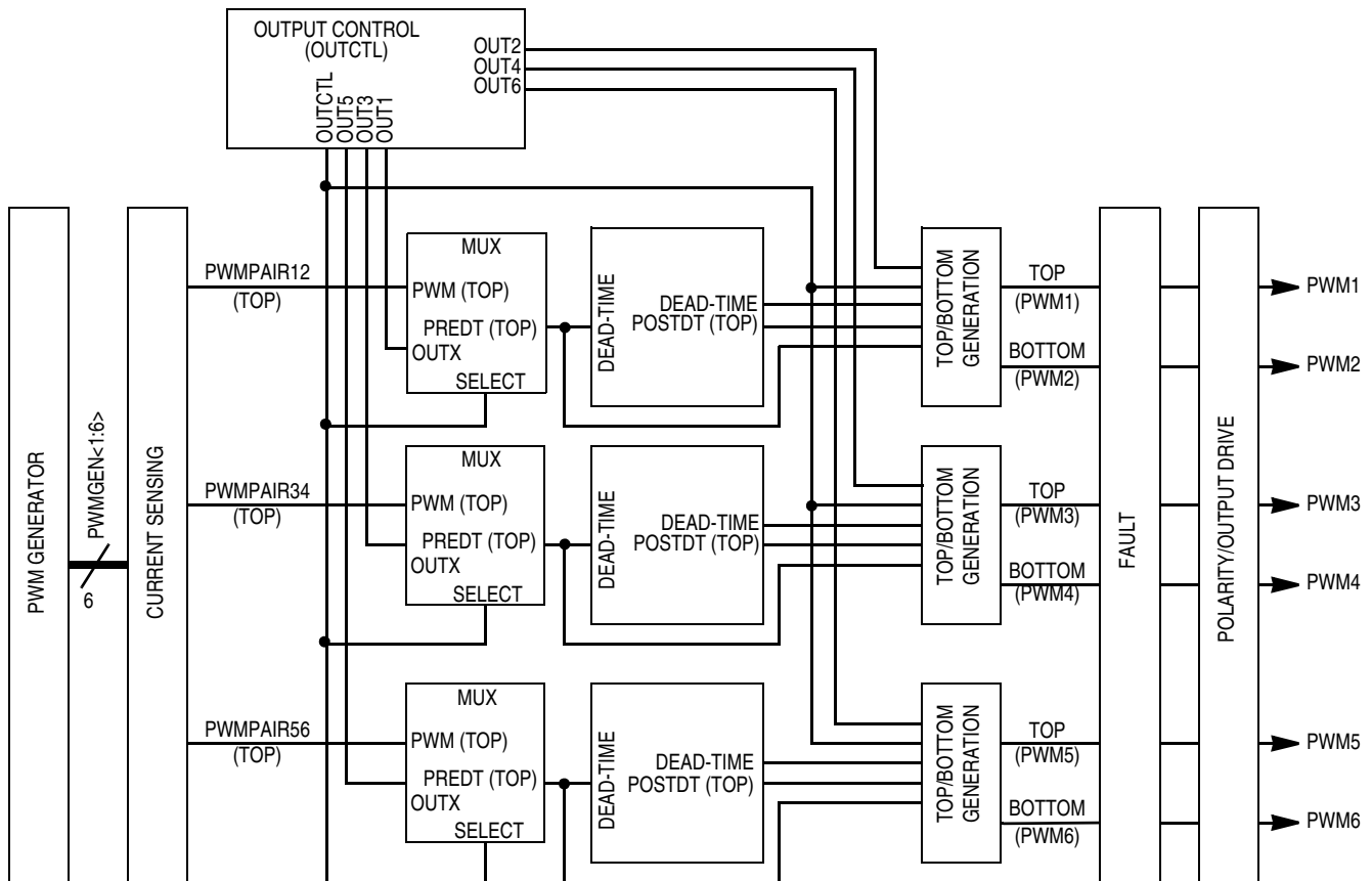
Figure 12-14. Dead-Time Generators
