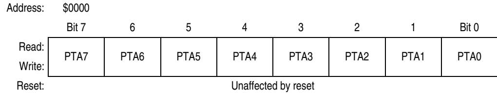
Figure 10-2. Port A Data Register (PTA)
