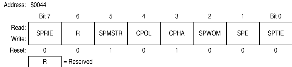
Figure 15-14. SPI Control Register (SPCR)
