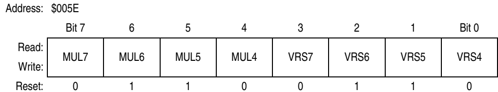
Figure 4-7. PLL Programming Register (PPG)
