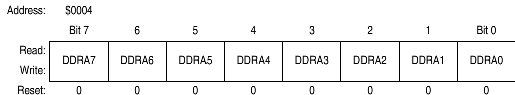
Figure 10-3. Data Direction Register A (DDRA)
