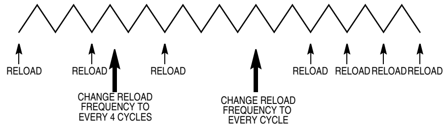
Figure 12-6. Reload Frequency Change
