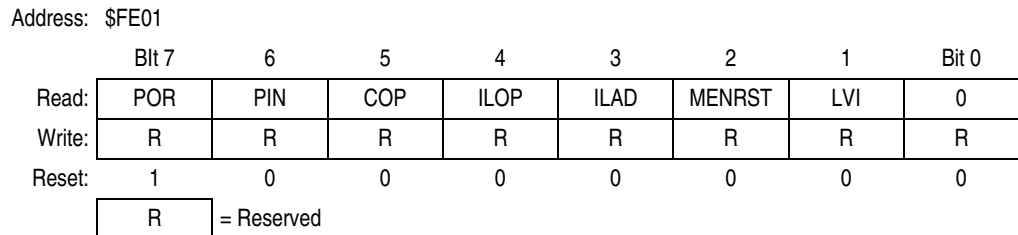
Figure 14-15. SIM Reset Status Register (SRSR)
