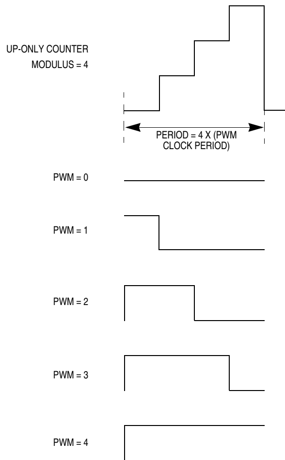
Figure 12-5. Edge-Aligned PWM (Positive Polarity)
