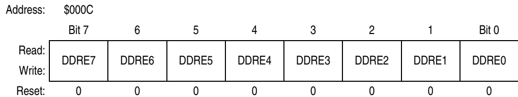
Figure 10-14. Data Direction Register E (DDRE)
