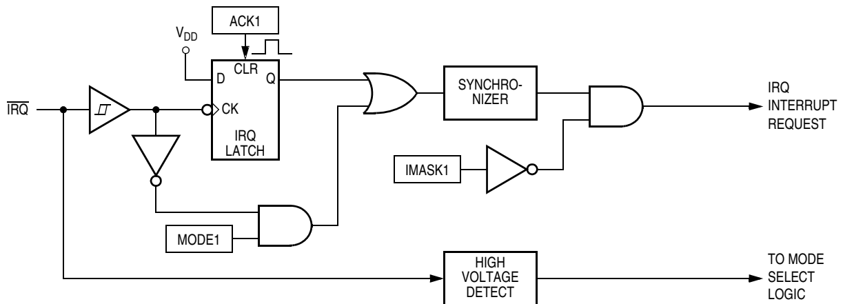
Figure 8-1. IRQ Module Block Diagram
