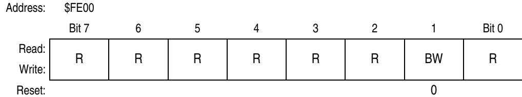
Figure 18-6. SIM Break Status Register (SBSR)
