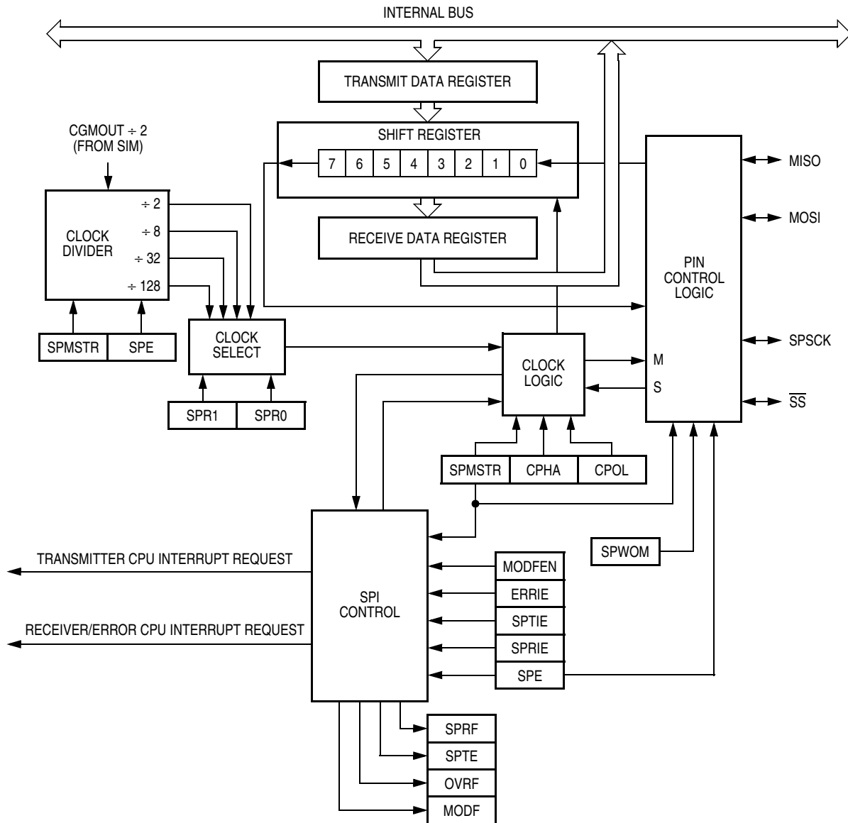
Figure 15-3. SPI Module Block Diagram
