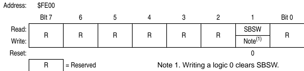
Figure 14-14. SIM Break Status Register (SBSR)
