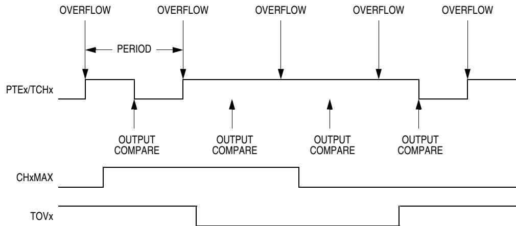
Figure 17-9. CHxMAX Latency
