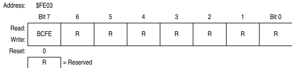
Figure 14-16. SIM Break Flag Control Register (SBFCR)
