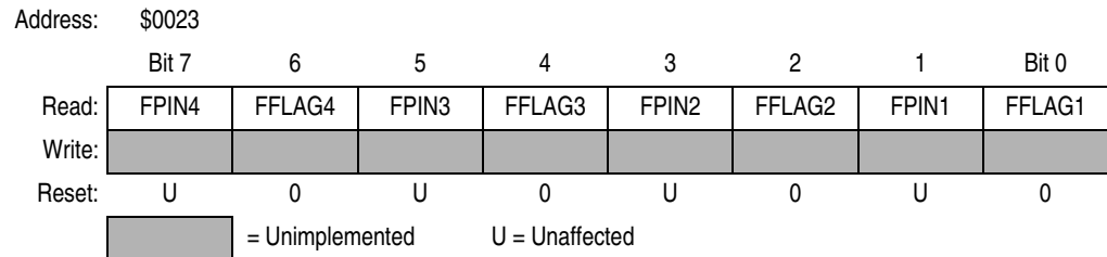
Figure 12-44. Fault Status Register (FSR)
