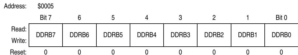
Figure 10-6. Data Direction Register B (DDRB)
