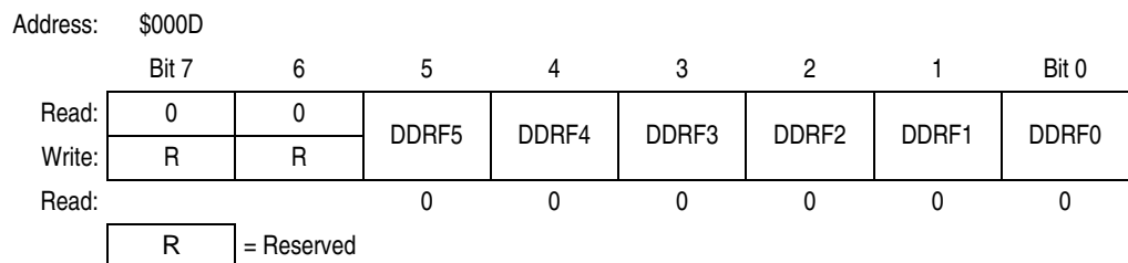
Figure 10-17. Data Direction Register F (DDRF)
