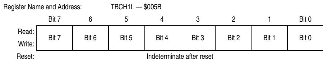
Figure 17-10. TIMB Channel Registers (TBCH0H/L–TBCH1H/L)
