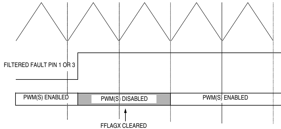
Figure 12-29. PWM Disabling in Manual Mode (Example 1)
