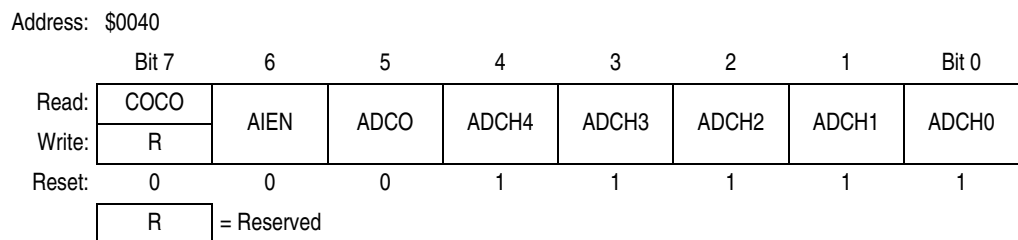
Figure 3-4. ADC Status and Control Register (ADSCR)
