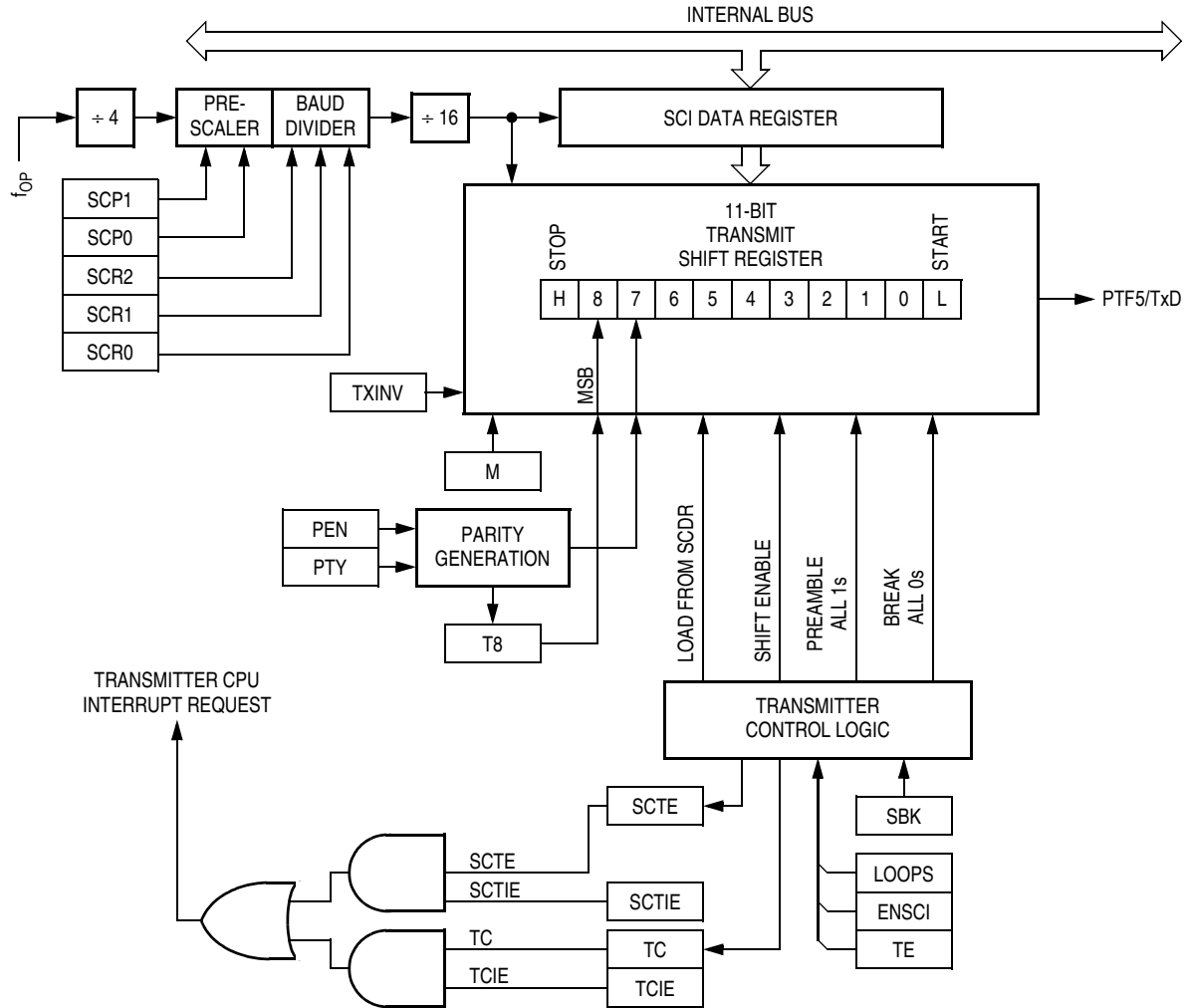
Figure 13-5. SCI Transmitter
