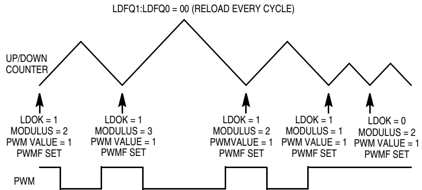
Figure 12-9. Center-Aligned Loading of Modulus
