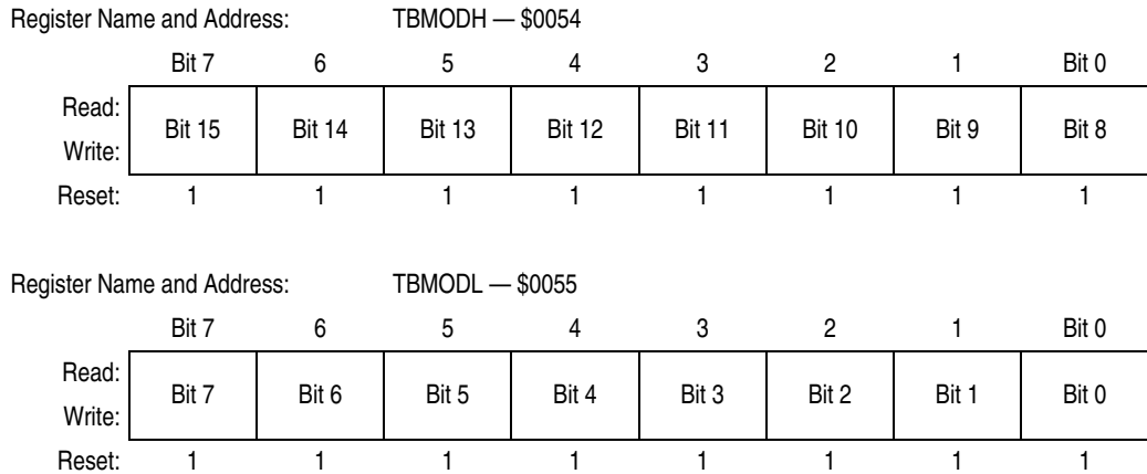
Figure 17-7. TIMB Counter Modulo Registers (TBMODH and TBMODL)
