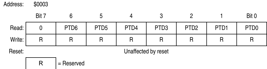
Figure 10-11. Port D Data Register (PTD)
