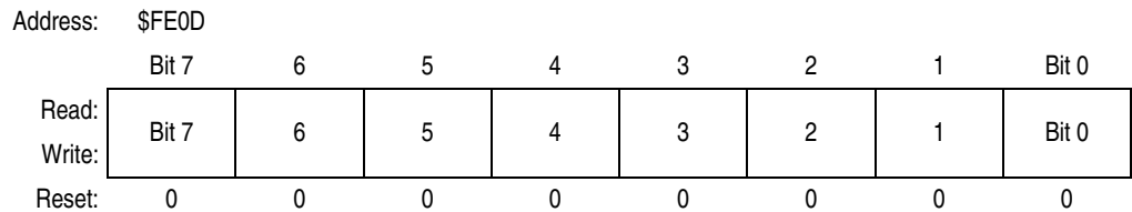
Figure 18-5. Break Address Register Low (BRKL)
