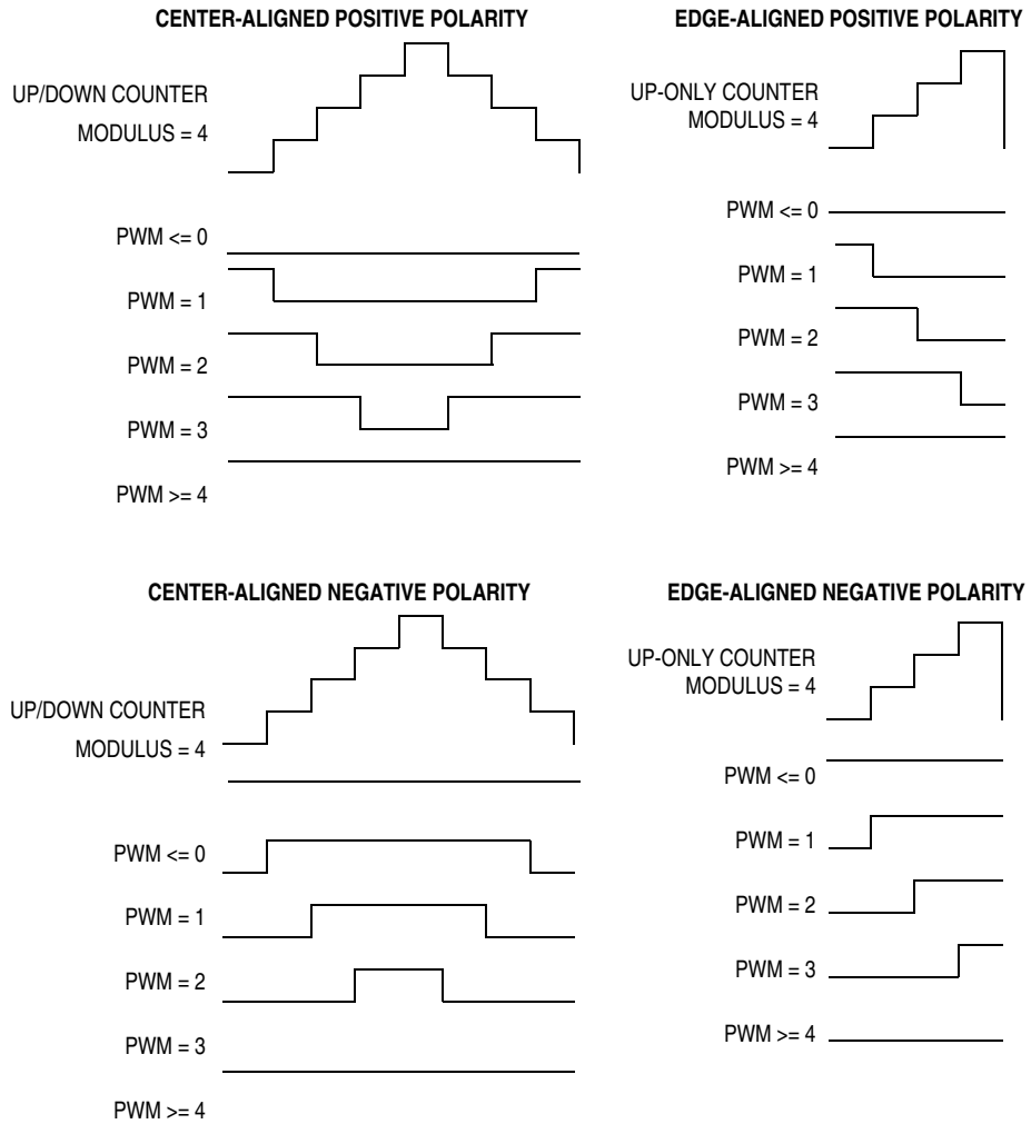
Figure 12-21. PWM Polarity
