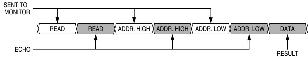
Figure 18-11. Read Transaction
