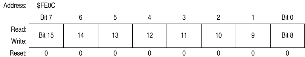
Figure 18-4. Break Address Register High (BRKH)
