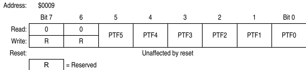
Figure 10-16. Port F Data Register (PTF)
