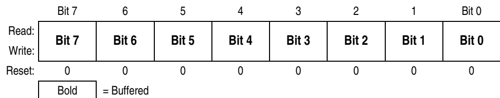
Figure 12-38. PWMx Value Registers Low (PVALxL)
