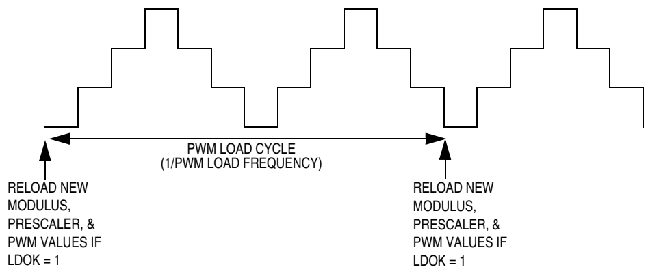
Figure 12-48. PWM Load Cycle/Frequency Definition
