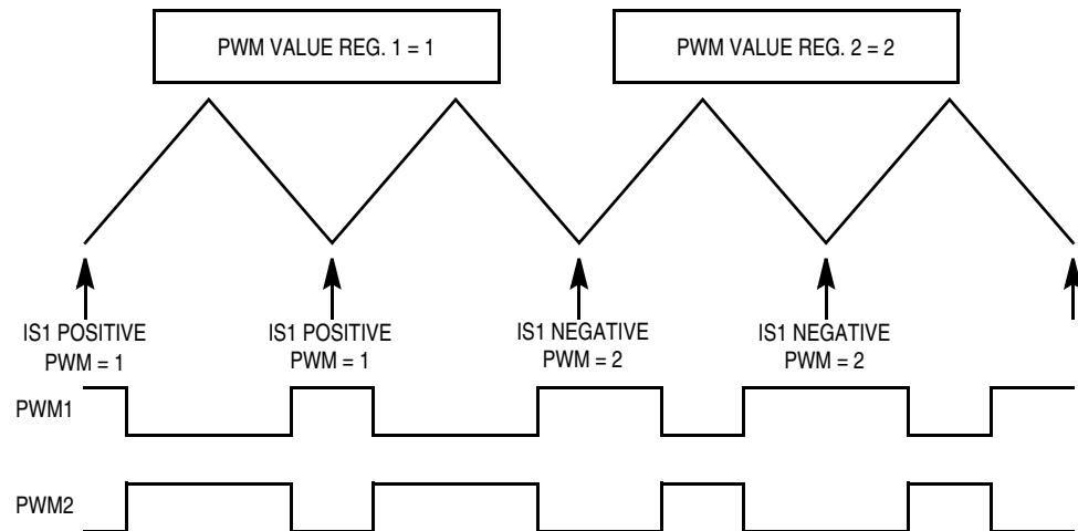
Figure 12-20. Top/Bottom Correction for PWMs 1 and 2
