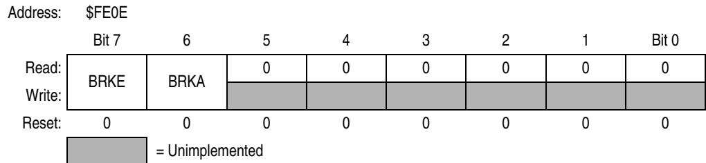
Figure 18-3. Break Status and Control Register (BRKSCR)
