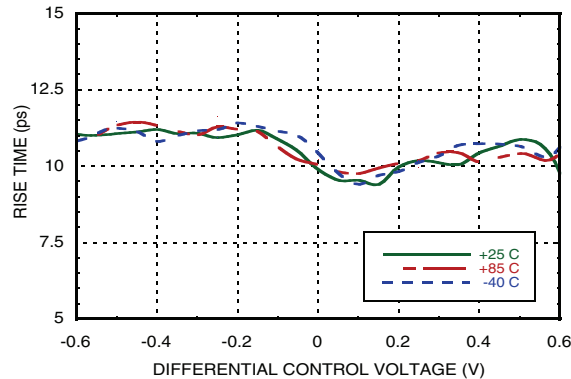
Rise Time vs. Temperature @ 16 GHz [1][4][5]
