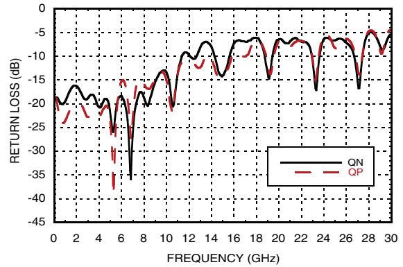
Output Return Loss vs. Frequency [1][3]
