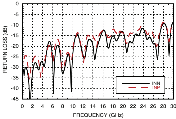
Input Return Loss vs. Frequency [1][3]
