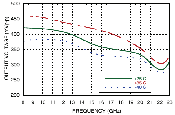
Single-Ended Output Swing vs. Frequency [1][2][3][4]
