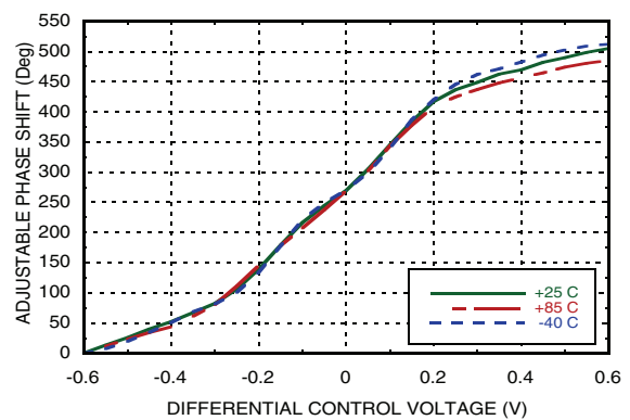
Phase Shift vs. Temperature [1][2][3][4]
