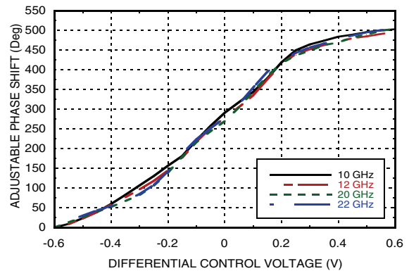
Phase Shift vs. Frequency [1][2][3]
