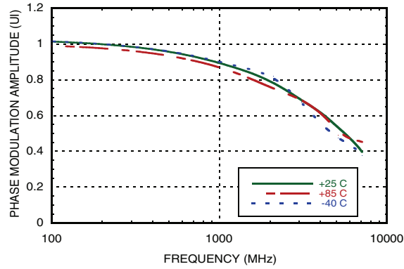
Modulation Signal Bandwidth vs. Temperature [1][2][7]
