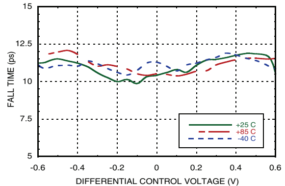
Fall Time vs. Temperature @ 16 GHz [1][4][5]
