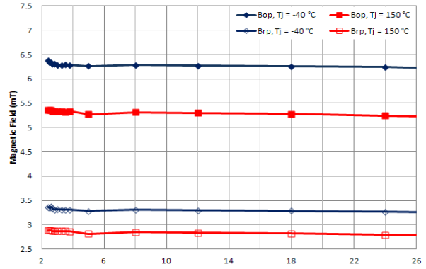
7.2 B_{OP} and B_{RP} vs. V_{DD}
