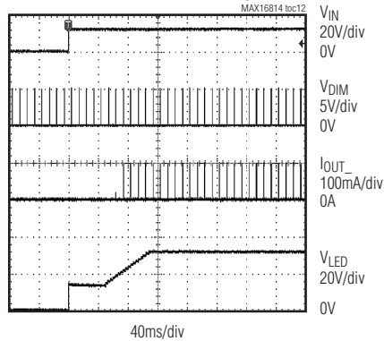
STARTUP WAVEFORM WITH DIM ON PULSE WIDTH < t sw
