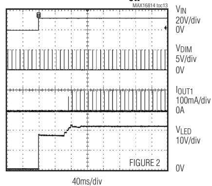
STARTUP WAVEFORM WITH DIM ON PULSE WIDTH = 10t sw
