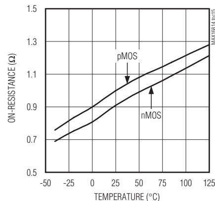
MOSFET DRIVER ON-RESISTANCE vs. TEMPERATURE
