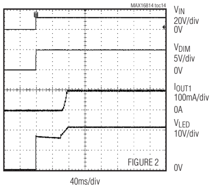
STARTUP WAVEFORM WITH DIM CONTINUOUSLY ON
