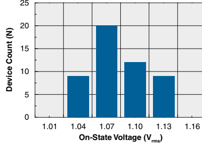
Typical On-State Voltage Distribution ( I_L=1\text{A}_{\text{rms}} , T_A=25^\circ\text{C} )
