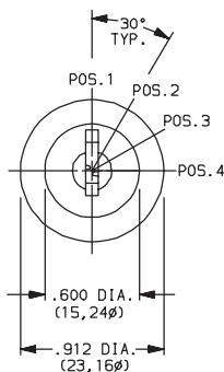
AX161X SWITCH FUNCTION SHOWN
