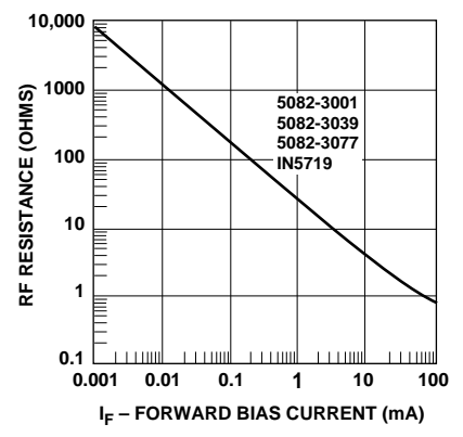
Figure 2. Typical RF Resistance vs. Forward Bias Current.
