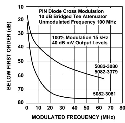
Figure 8. Typical Cross Intermodulation Distortion.
