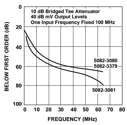
Figure 7. Typical Second Order Intermodulation Distortion.
