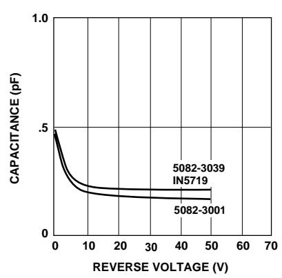
Figure 4. Typical Capacitance vs. Reverse Voltage.
