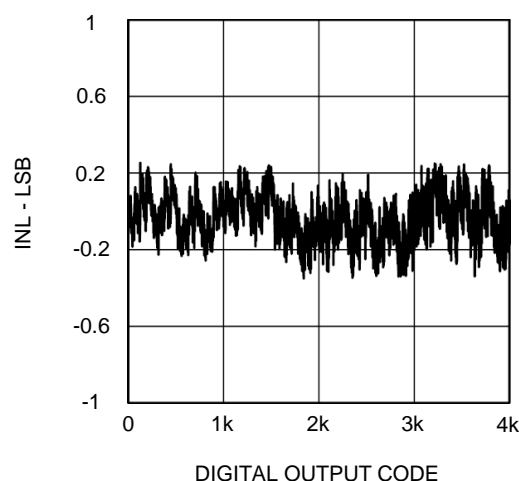
Integral Nonlinearity
