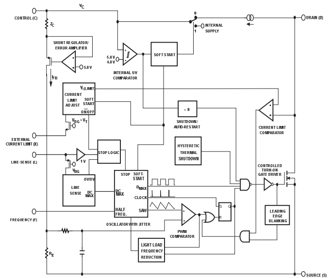
TOP249 BLOCK DIAGRAM
