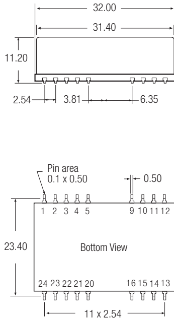
SMD Package Style
