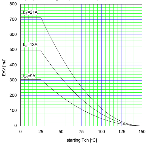
Maximum Avalanche Energy vs. starting T ch E(AV)=f(\text{starting } T_{ch}):V_{cc}=50V, I(AV)\leq 21A
