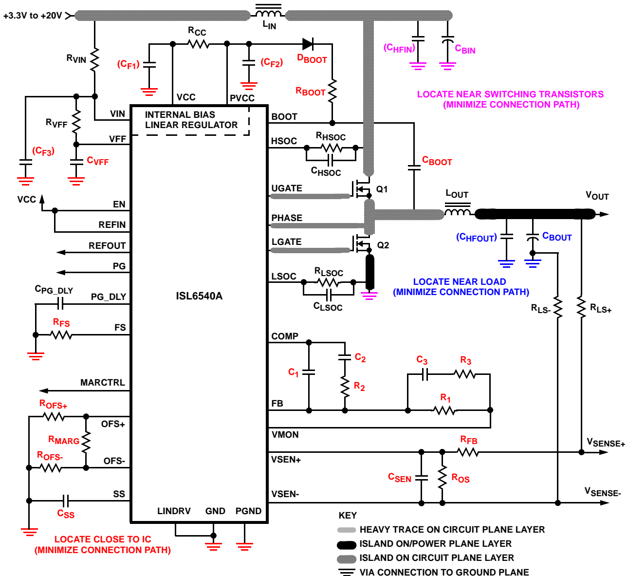
FIGURE 7. PRINTED CIRCUIT BOARD POWER PLANES AND ISLANDS
