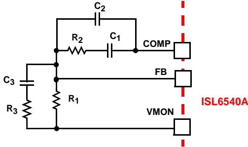
FIGURE 8. COMPENSATION CONFIGURATION FOR ISL6540A WHEN USING DIFFERENTIAL REMOTE SENSE
