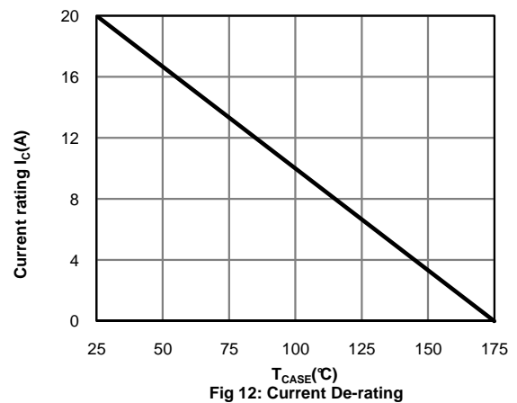
Fig 12: Current De-rating
