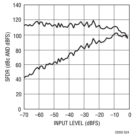
LTC2203: SFDR vs Input Level, f_{IN} = 30.1\text{MHz} , PGA = 0, Dither "On"
