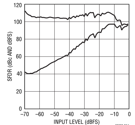
LTC2202: SFDR vs Input Level, f IN = 12.4MHz, PGA = 0, Dither "Off"
