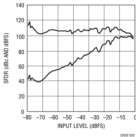
LTC2203: SFDR vs Input Level, f_{IN} = 30.1\text{MHz} , PGA = 0, Dither "Off"
