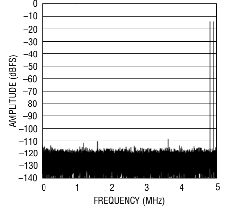
LTC2202: 32K Point 2-Tone FFT, f IN = 5.1MHz and 15.2MHz, -15dBFS, PGA = 0
