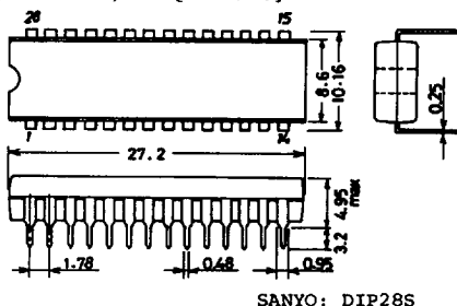
Case Outline 3029A (unit : mm) [LC7523]
