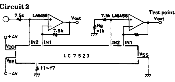
Test Circuit 2
