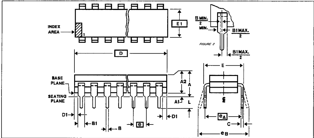
24 PINS CERP .600
