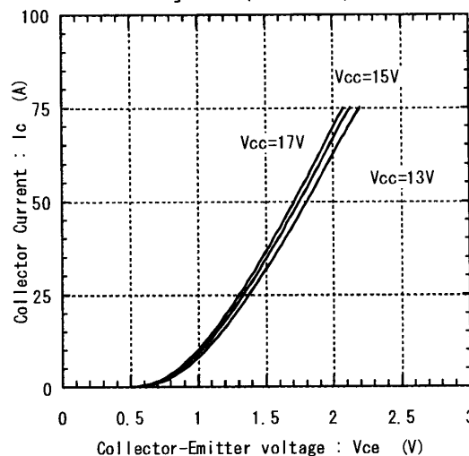
Collector current vs. Collector-Emmitter voltage T_j=25^\circ\text{C} (Terminal)
