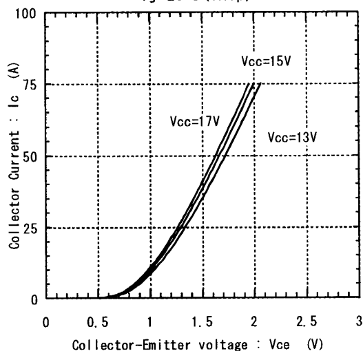
Collector current vs. Collector-Emmitter voltage T_j=25^\circ\text{C} (Chip)
