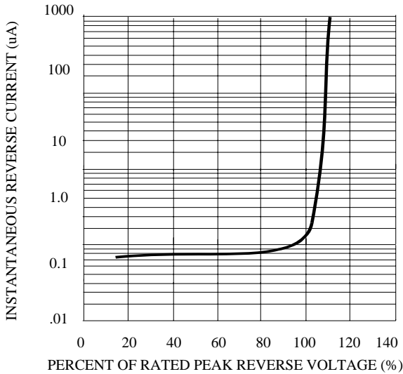
FIG. 3-TYPICAL REVERSE CHARACTERISTICS
