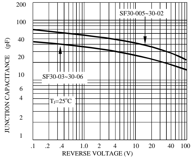
FIG. 6-TYPICAL JUNCTION CAPACITANCE
