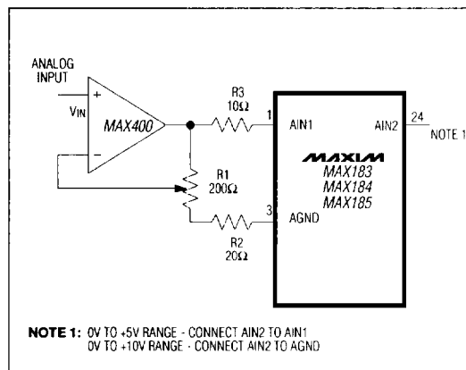
Figure 18. Unipolar Operation with Gain Adjust
