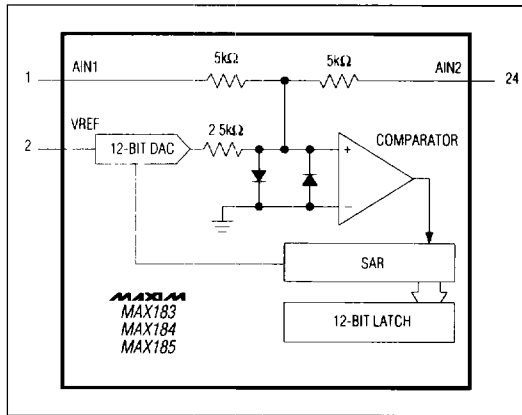
Figure 4. MAX183/184/185 AIN Inputs
