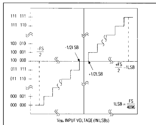
Figure 20. Ideal Input/Output Transfer Characteristic for Bipolar Operation
