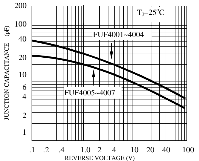
FIG. 6-TYPICAL JUNCTION CAPACITANCE
