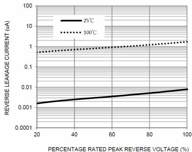
FIG. 4-TYPICAL REVERSE CHARACTERISTICS
