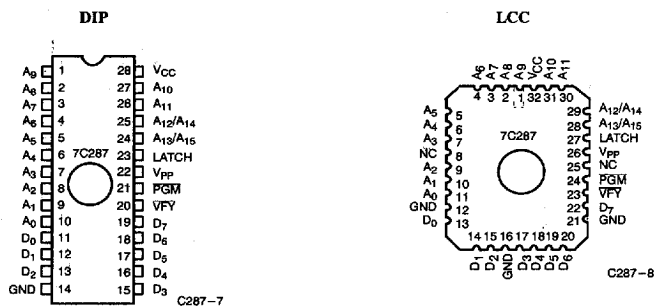
Figure 1. Programming Pinouts
