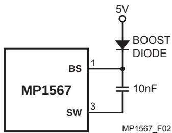
Figure 2—External Boost Diode
