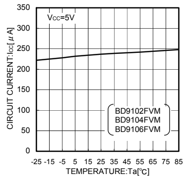
Fig.35 Ta-Icc
