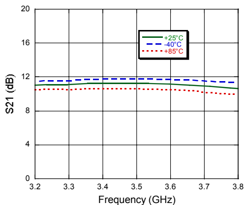
Gain
