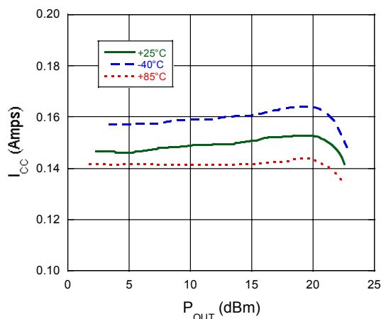
I_{CC} vs. P_{OUT} @ 2140 MHz
