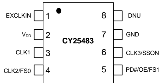
Figure 2. Pin Diagram - CY25483 8-Pin SOIC
