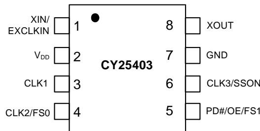
Figure 1. Pin Diagram - CY25403 8-Pin SOIC
