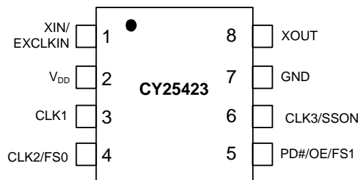
Figure 3. Pin Diagram - CY25423 8-Pin SOIC
