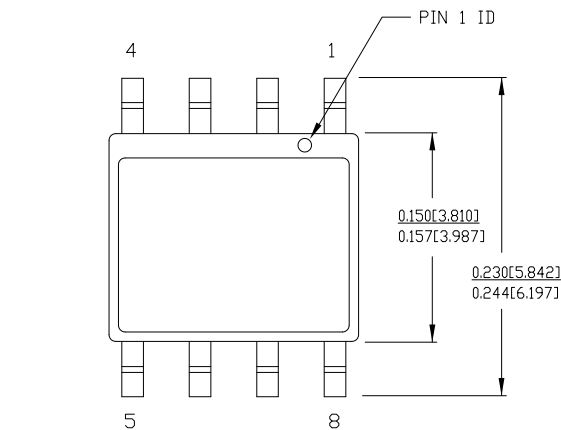
Figure 7. 8-Pin (150-Mil) SOIC S8
