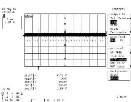
Ref.8-1 PC V Signal input : IC501, #182
