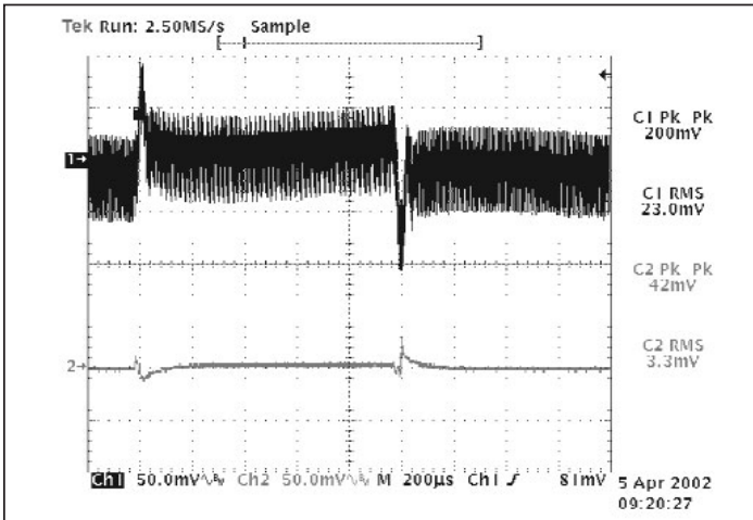
Figure 15 —V48C5C100A and μRAM; Input and output dynamic response no added C TRAN ; 22.5% of 20A rating load step of 4.5A (10A →14.5A);RHR=31k (Configured as in Figs. 1 & 2)
