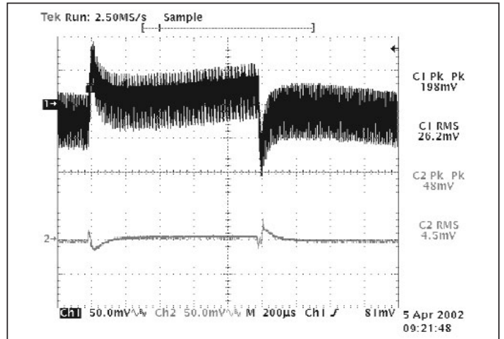
Figure 16 —V48C5C100A and μRAM; Input and output dynamic response C TRAN =820μF Electrolytic; 35% of load step of 7A (10A →17A);RHR=31k (Configured as in Figs. 1 & 2)
