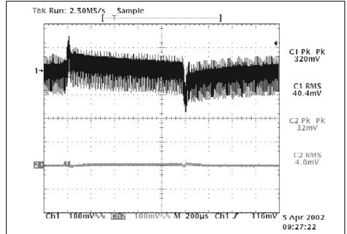
Figure 12 —V300B12C250A and μRAM; Input and output dynamic response no added C TRAN ; 17.5% of 20A rating load step of 3.5A (10A →13.5A);RHR=80k (Configured as in Figs. 1 & 2)
