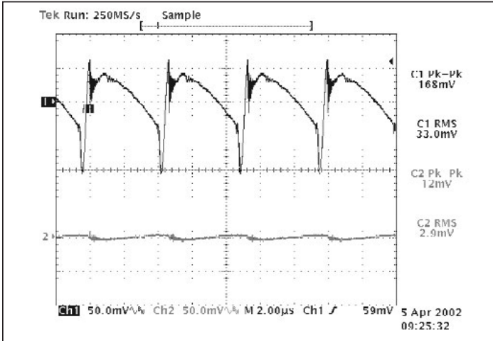
Figure 11 —V375B12C250A and μRAM; Input and output ripple @50% (10A) load CH1=Vi; CH2=Vo; Vi-Vo=305mV; RHR=80k (Configured as in Figs. 1 & 2)
