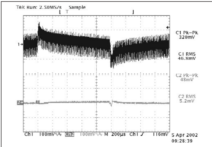
Figure 13 —V300B12C250A and μRAM; Input and output dynamic response C TRAN =820μF Electrolytic; 30% of load step of 6A (10A →16A);RHR=80k (Configured as in Figs. 1 & 2)
