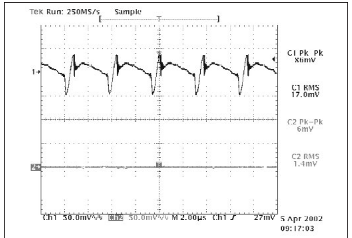
Figure 14 —V48C5C100A and μRAM; Input and output ripple @50% (10A) load CH1=Vi; CH2=Vo; Vi-Vo=327mV; RHR=31k (Configured as in Figs. 1 & 2)
