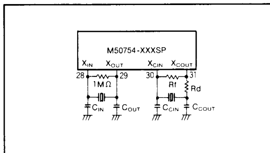
Fig.21 Example ceramic resonator circuit
