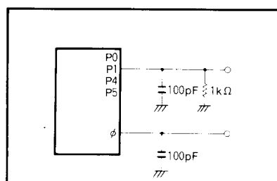
Fig.27 Port P0, P1, P4, P5 test circuit
