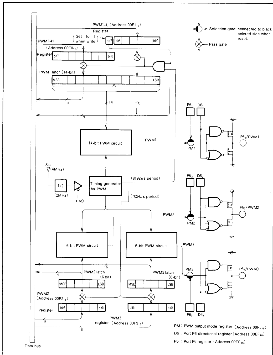
Fig.9 Block diagram of the PWM circuit
