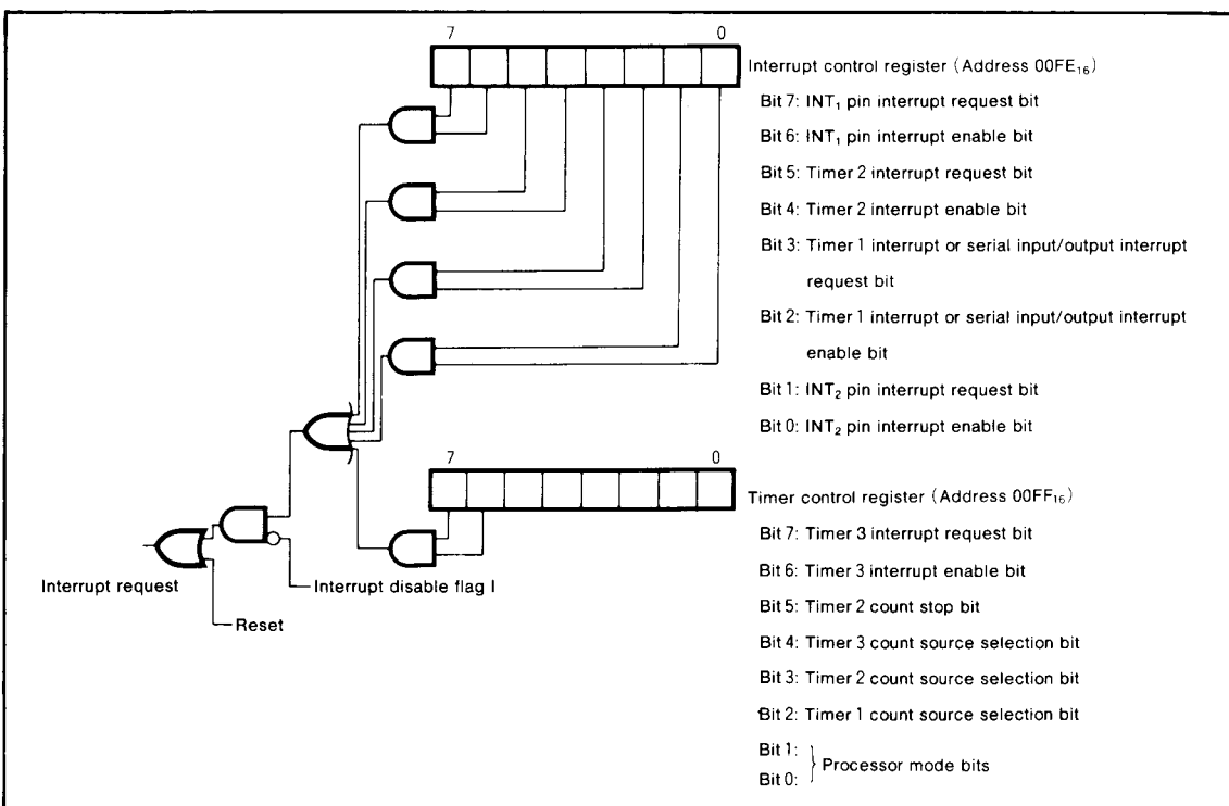
Fig.3 Interrupt control
