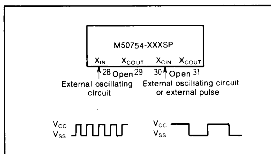
Fig.22 Example clock input circuit
