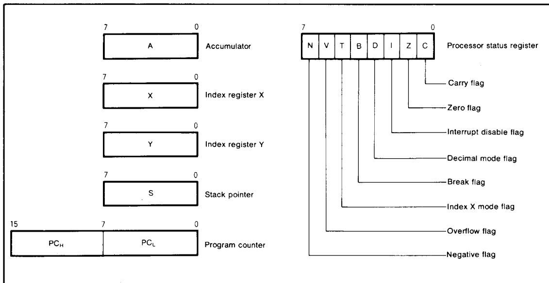
Fig.2 Register structure
