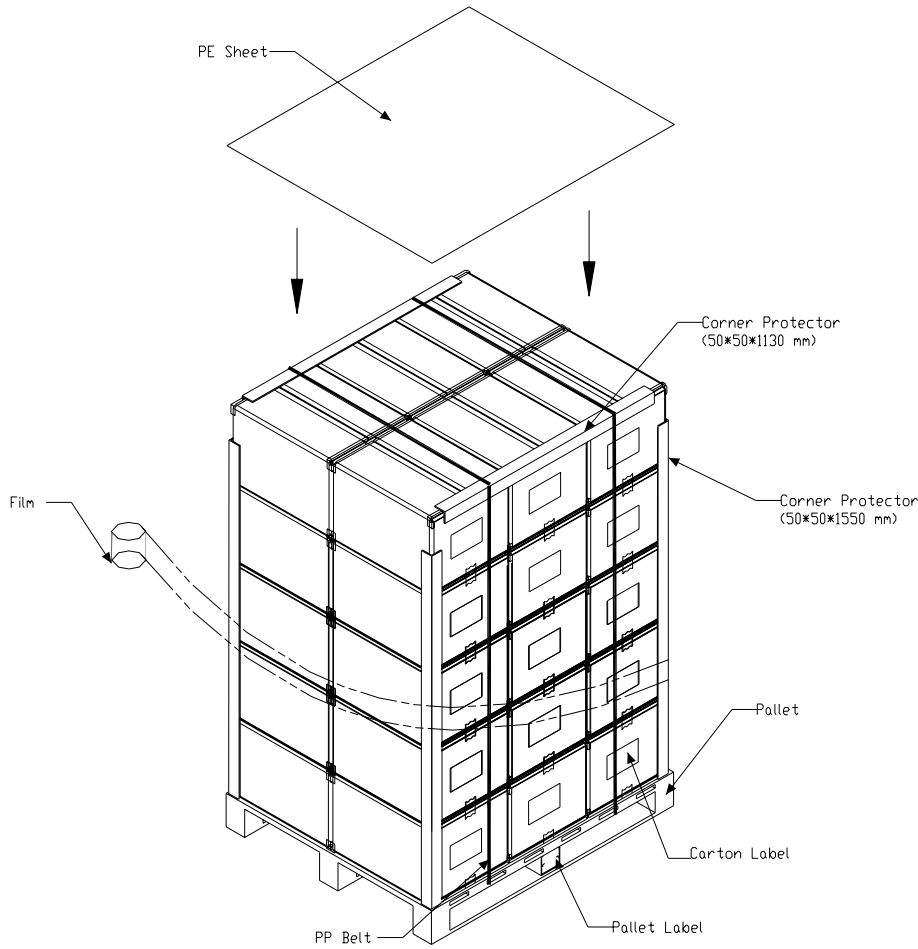
Figure. 9-2 Packing method
