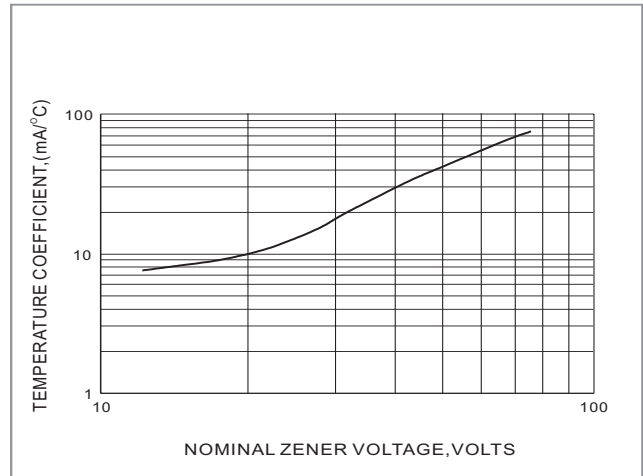
Fig.2 TEMPERATURE COEFFICIENTS
