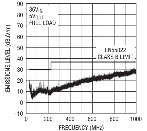
Radiated Emissions
