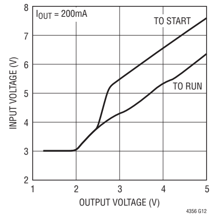
Minimum Required Input Voltage vs Output Voltage
