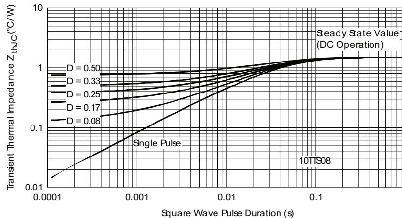
Fig. 8 - Thermal Impedance Z_{\theta JC} Characteristics
