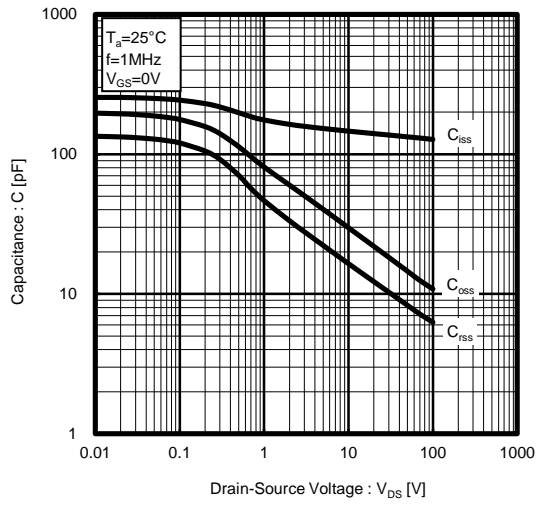
Fig.13 Typical Capacitance vs. Drain-Source Voltage
