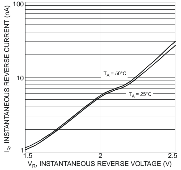
Fig. 4 Typical Reverse Characteristics - GDZ5V1LP3
