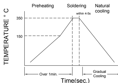
Figure 2. Hand Soldering
