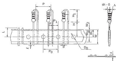
VT-Style (CFS 1/4 & MFS 1/4)
