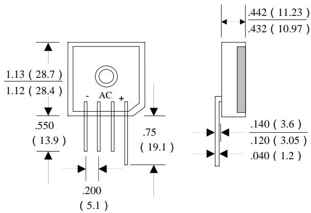
BP25-L IN LINE PIN CONFIGURATION (PLASTIC CASE)
