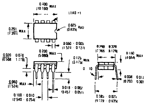
8 Lead CERDIP
