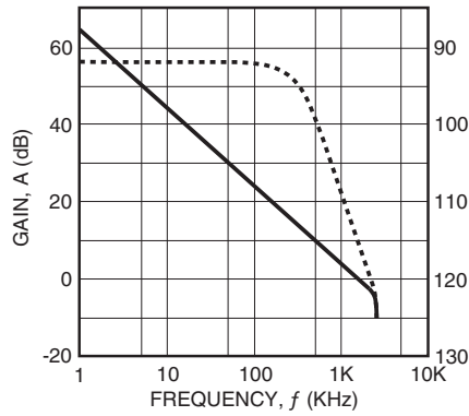
VOLTAGE GAIN & PHASE vs. FREQUENCY
